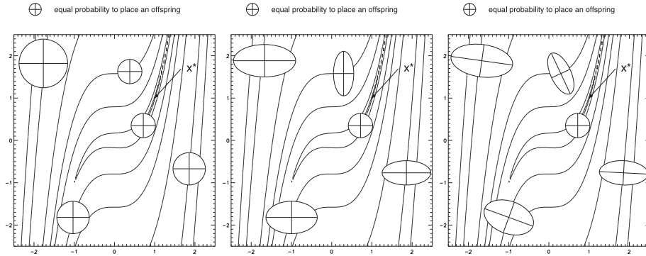
Figure 1.2: Equidensity probability contours for the three different approaches with respect to a 2D landscape. Left: A single global step-size (circles). Middle: n independent parameters (axis-parallel ellipsoids). Right: (n \cdot (n + 1)) / 2 independent parameters (arbitrarily oriented ellipsoids). Figures courtesy of Thomas Bäck [20].
